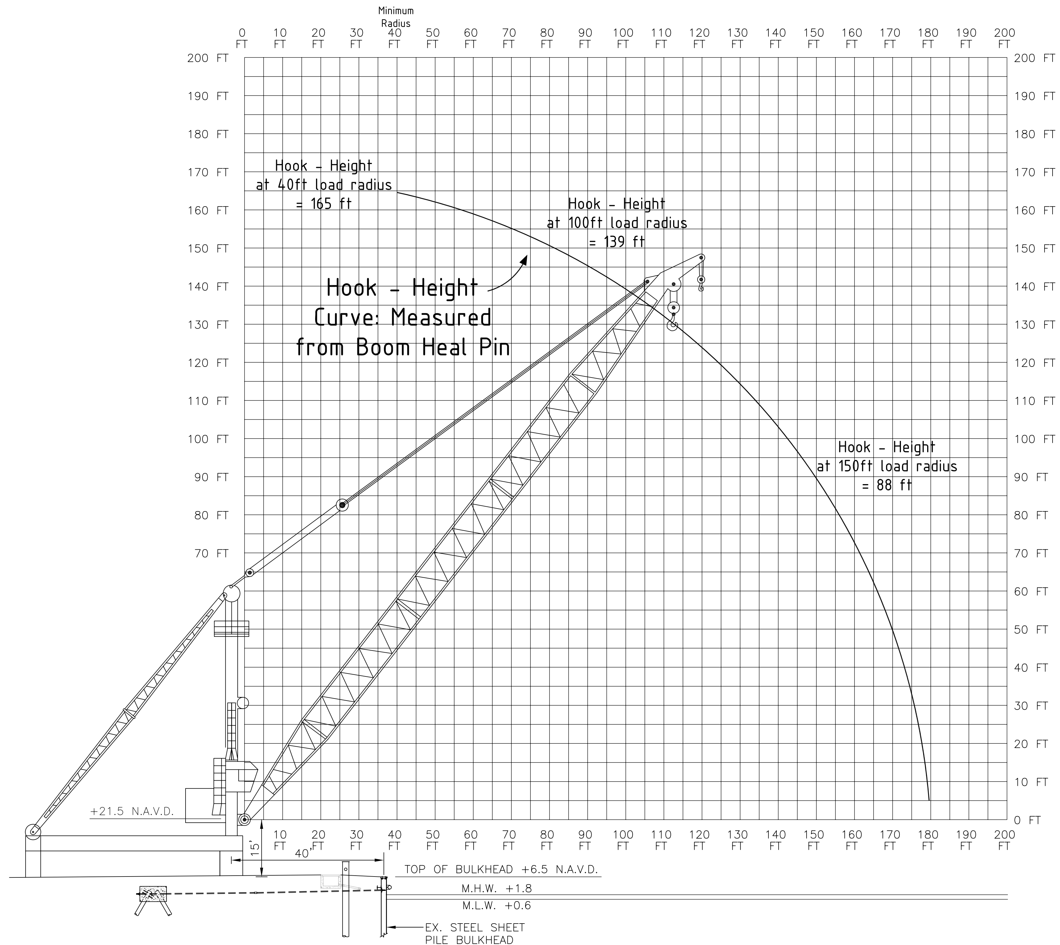
PROPOSED "300-TON" STIFFLEG CRANE (ELEV. VIEW) NOT TO SCALE
